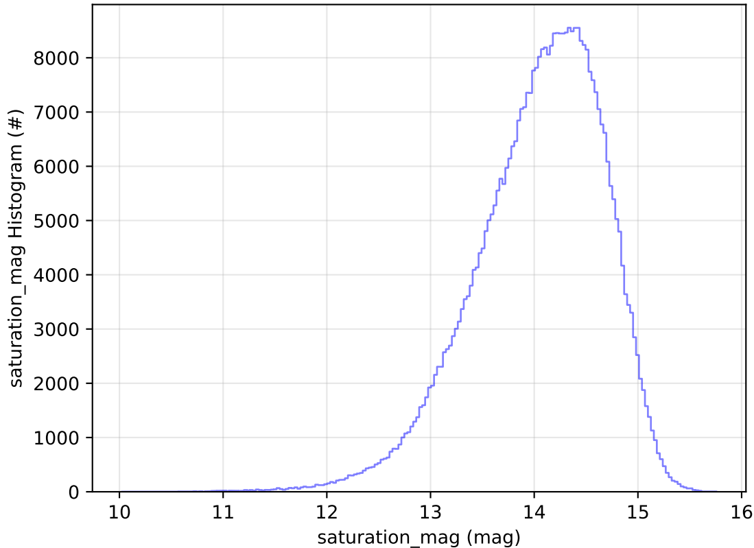
ddf_acor_sf25_lsf40_lsr10_v3.4_10yrs All sky z band: saturation_mag Histogram
