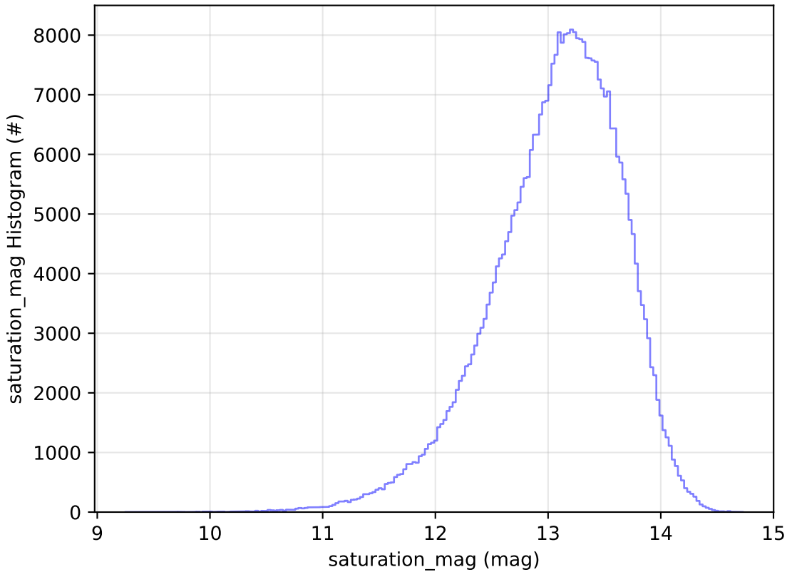
ddf_acor_sf25_lsf40_lsr10_v3.4_10yrs All sky y band: saturation_mag Histogram
