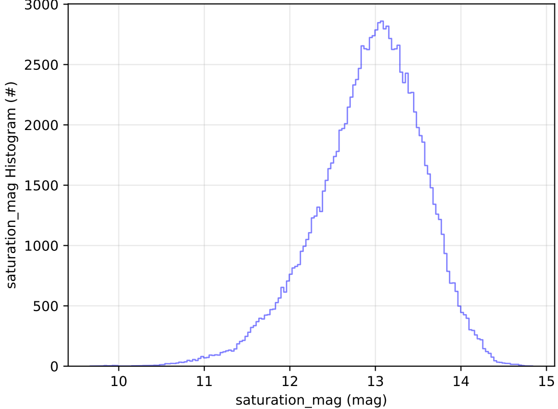
ddf_acor_sf25_lsf40_lsr10_v3.4_10yrs All sky u band: saturation_mag Histogram
