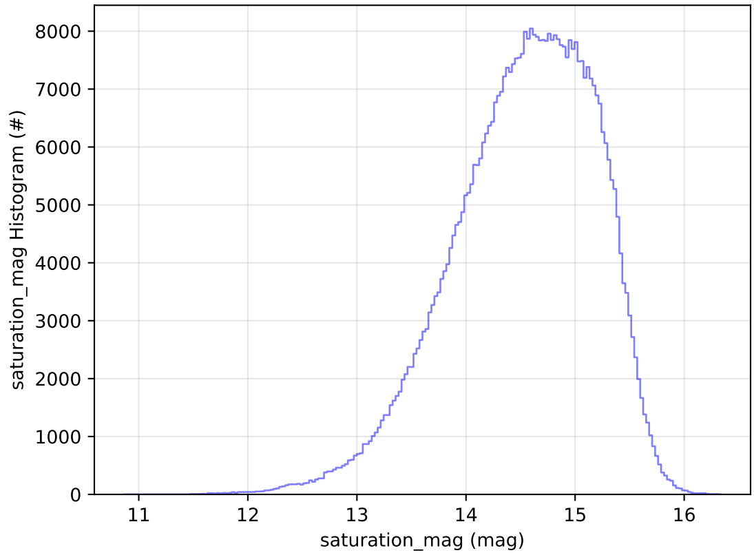
ddf_acor_sf25_lsf40_lsr10_v3.4_10yrs All sky r band: saturation_mag Histogram
