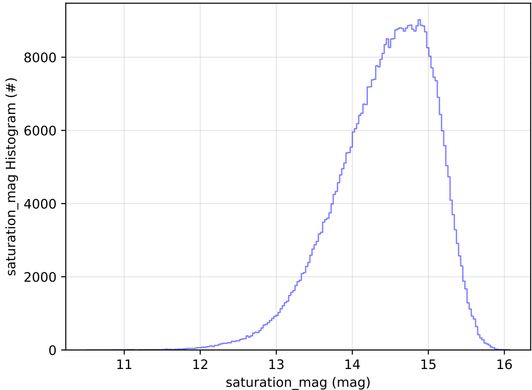
ddf_acor_sf25_lsf40_lsr10_v3.4_10yrs All sky i band: saturation_mag Histogram
