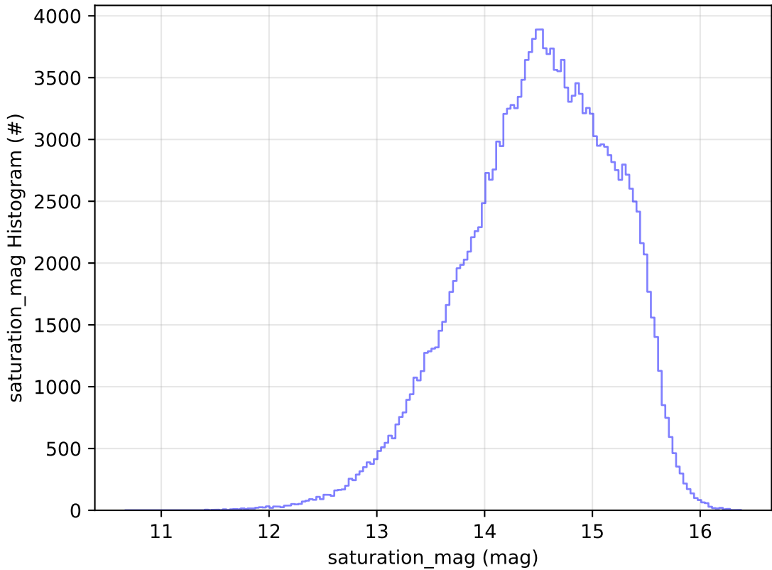
ddf_acor_sf25_lsf40_lsr10_v3.4_10yrs All sky g band: saturation_mag Histogram
