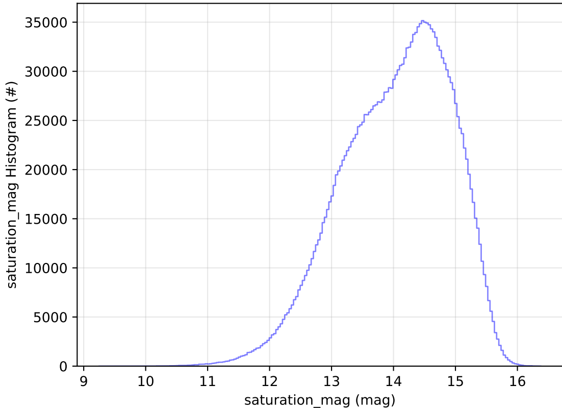
ddf_acor_sf25_lsf40_lsr10_v3.4_10yrs All sky all bands: saturation_mag Histogram
