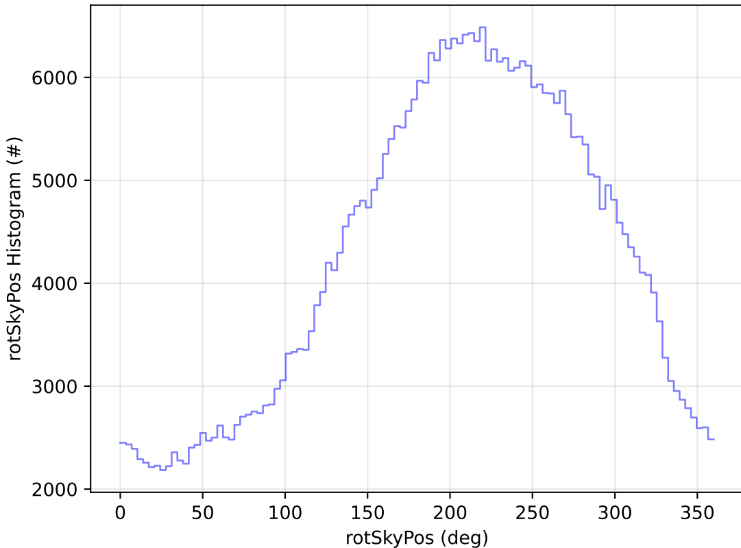
ddf_acor_sf25_lsf40_lsr10_v3.4_10yrs WFD z band: rotSkyPos Histogram
