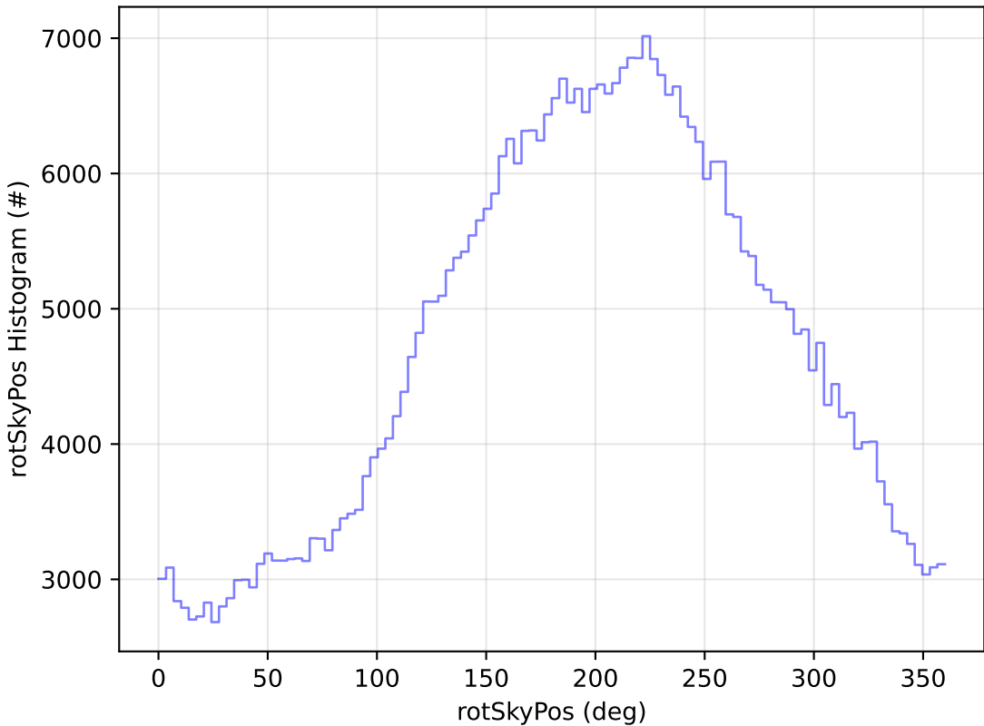
ddf_acor_sf25_lsf40_lsr10_v3.4_10yrs WFD r band: rotSkyPos Histogram
