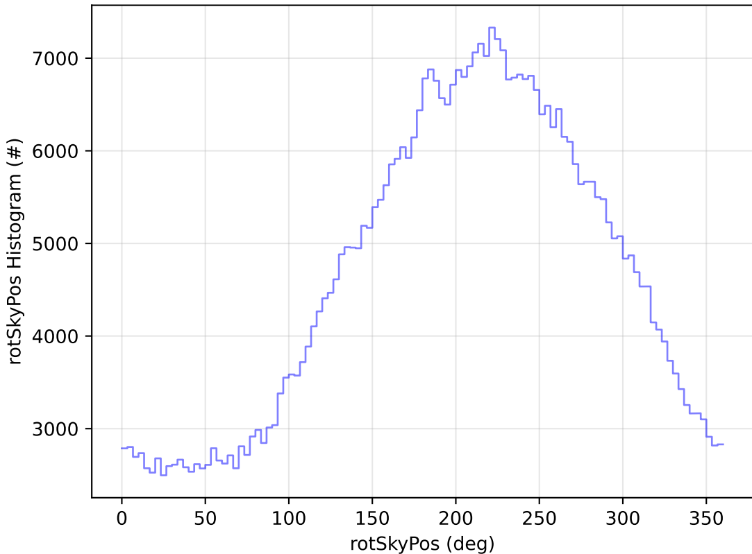
ddf_acor_sf25_lsf40_lsr10_v3.4_10yrs WFD i band: rotSkyPos Histogram
