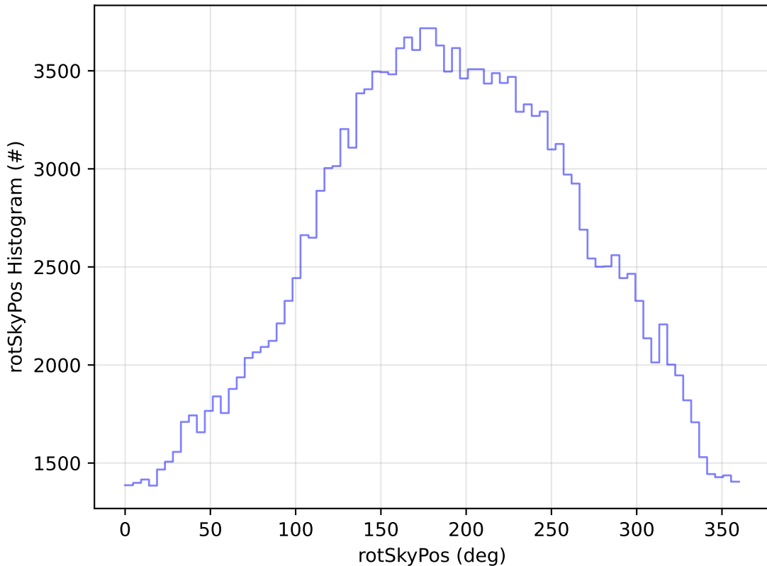
ddf_acor_sf25_lsf40_lsr10_v3.4_10yrs WFD g band: rotSkyPos Histogram
