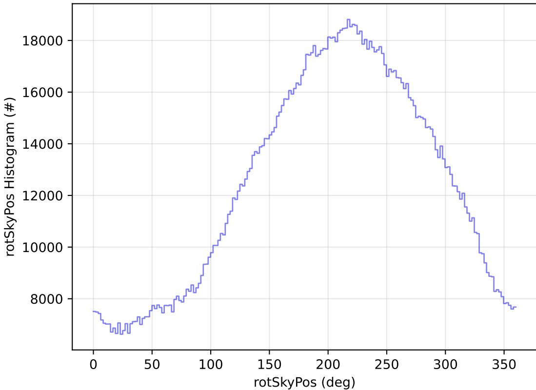
ddf_acor_sf25_lsf40_lsr10_v3.4_10yrs WFD all bands: rotSkyPos Histogram
