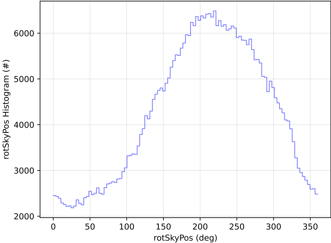
ddf_acor_sf25_lsf40_lsr10_v3.4_10yrs All sky z band: rotSkyPos Histogram
