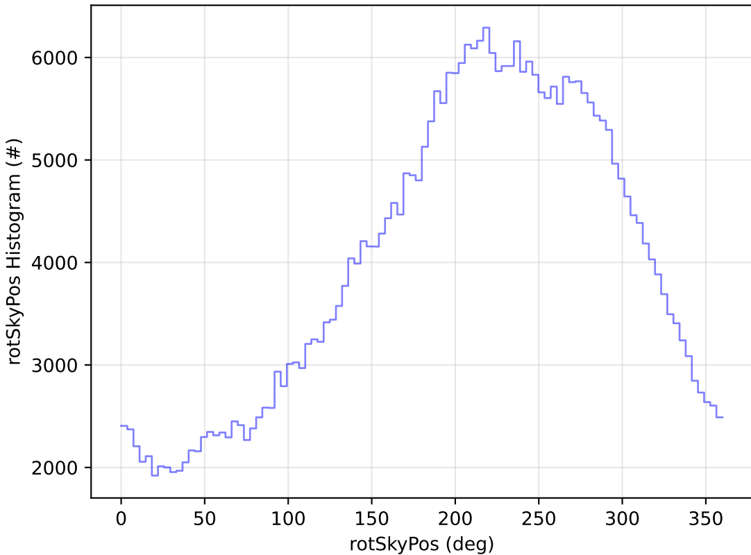
ddf_acor_sf25_lsf40_lsr10_v3.4_10yrs All sky y band: rotSkyPos Histogram
