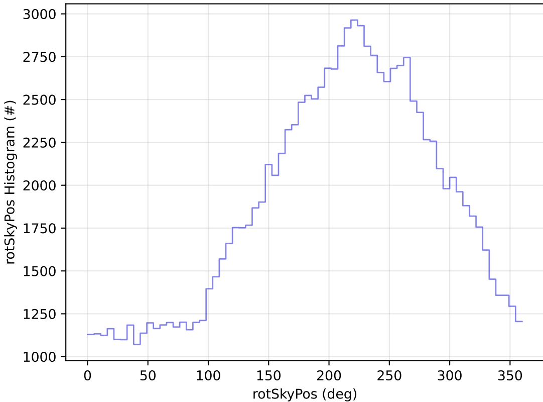
ddf_acor_sf25_lsf40_lsr10_v3.4_10yrs All sky u band: rotSkyPos Histogram
