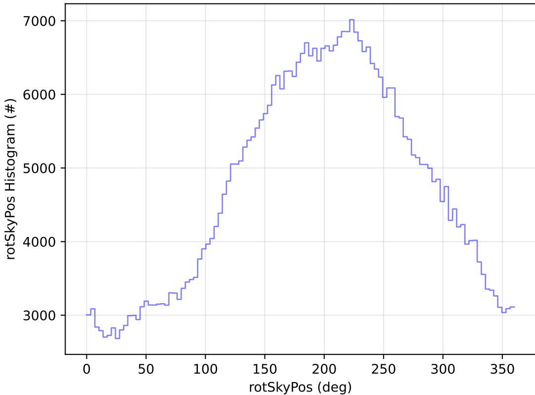
ddf_acor_sf25_lsf40_lsr10_v3.4_10yrs All sky r band: rotSkyPos Histogram
