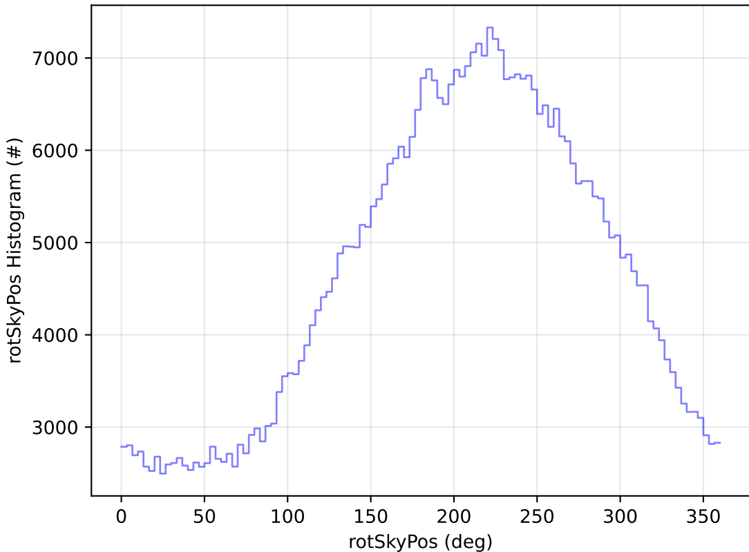
ddf_acor_sf25_ls40_lsr10_v3.4_10yrs All sky i band: rotSkyPos Histogram
