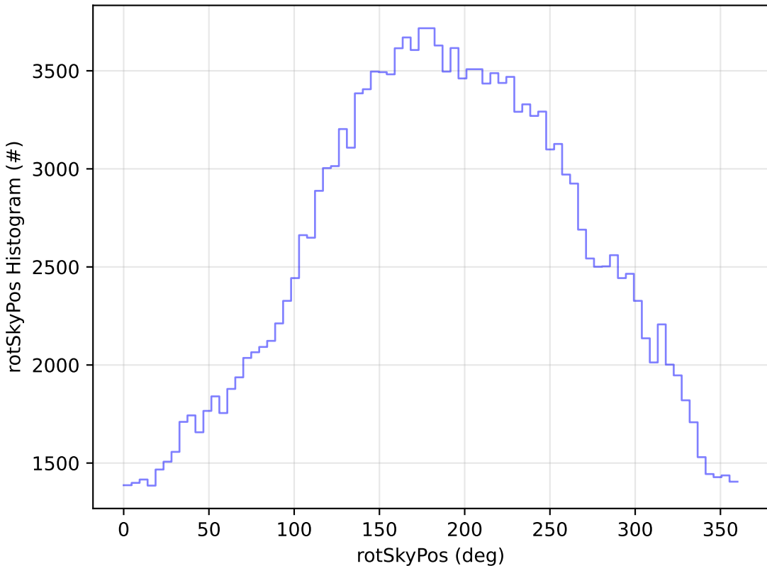
ddf_acor_sf25_lsf40_lsr10_v3.4_10yrs All sky g band: rotSkyPos Histogram
