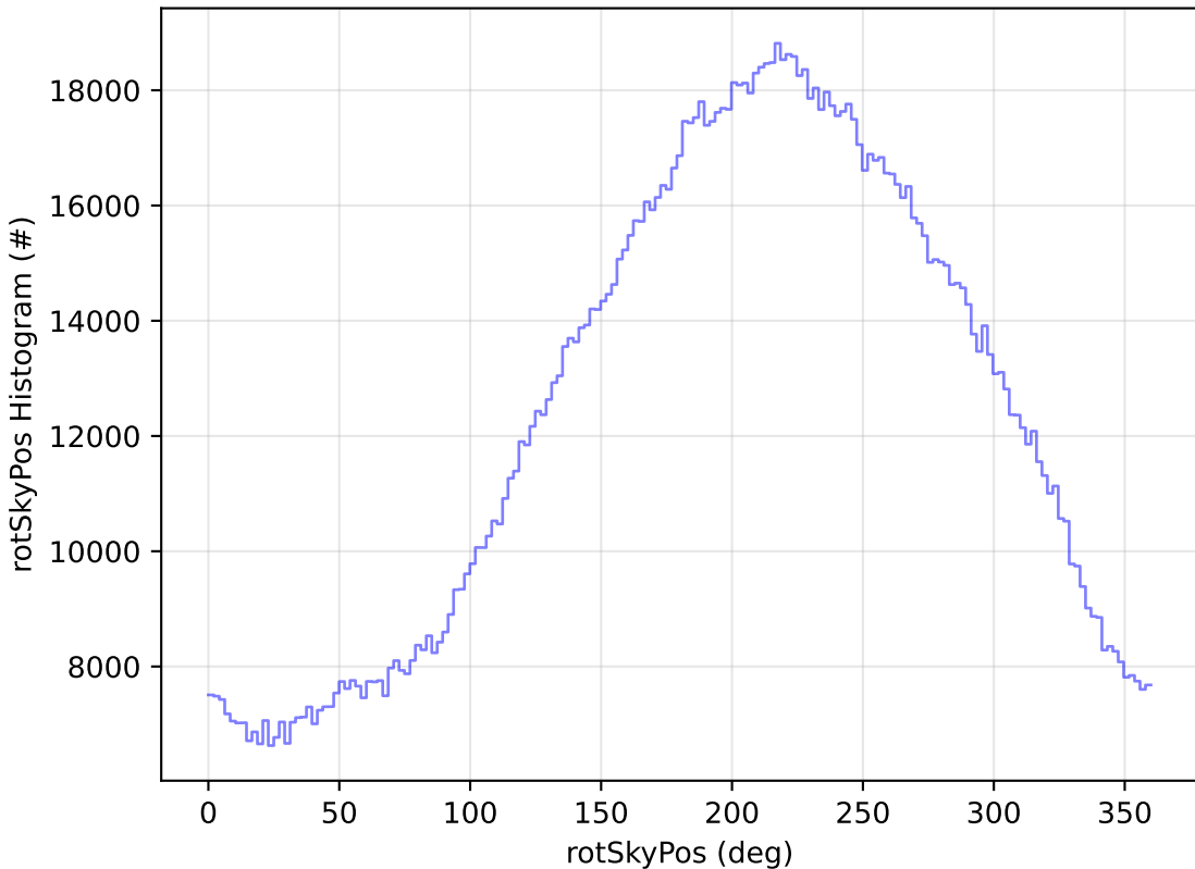
ddf_acor_sf25_lsf40_lsr10_v3.4_10yrs All sky all bands: rotSkyPos Histogram
