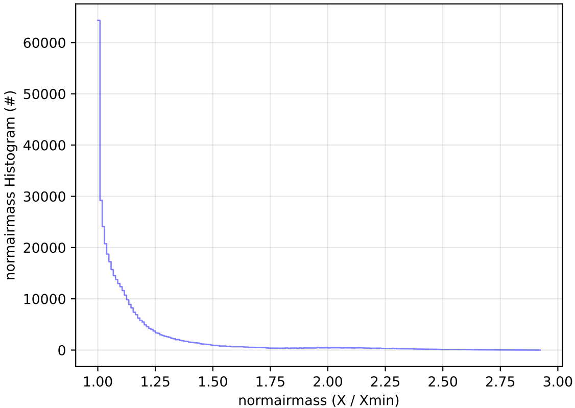
ddf_acor_sf25_lsf40_lsr10_v3.4_10yrs WFD z band: normairmass Histogram
