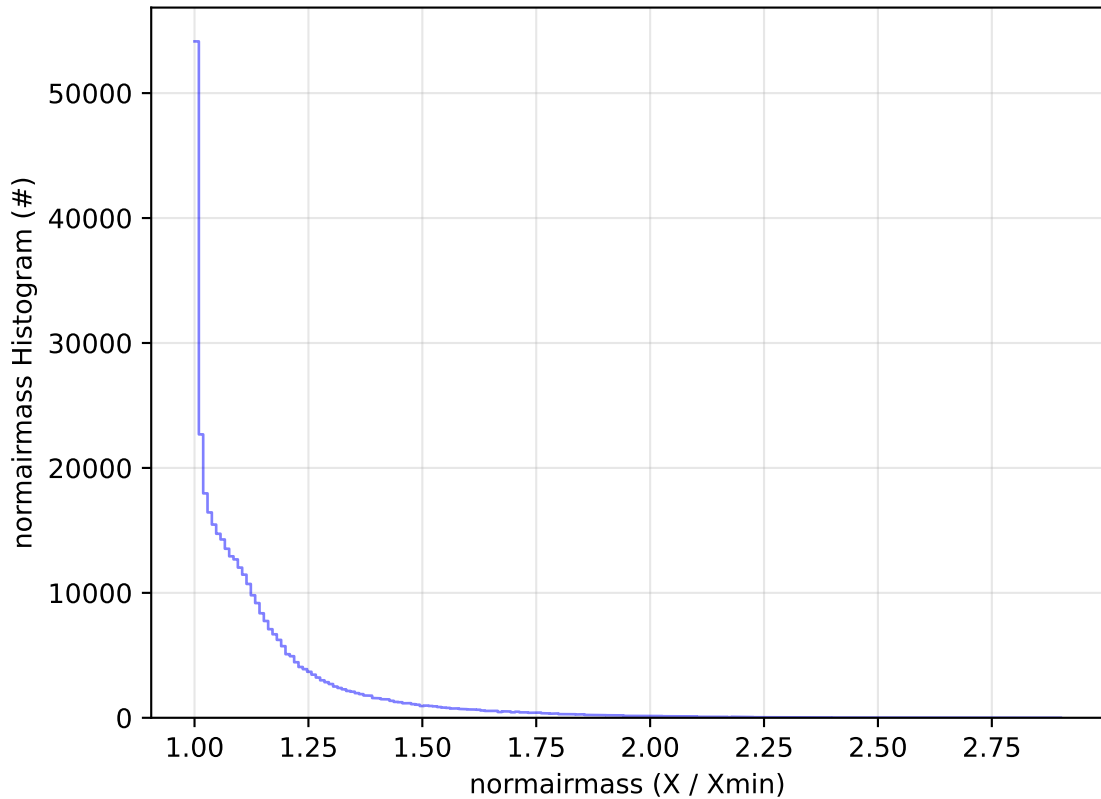
ddf_acor_sf25_lsf40_lsr10_v3.4_10yrs WFD y band: normairmass Histogram
