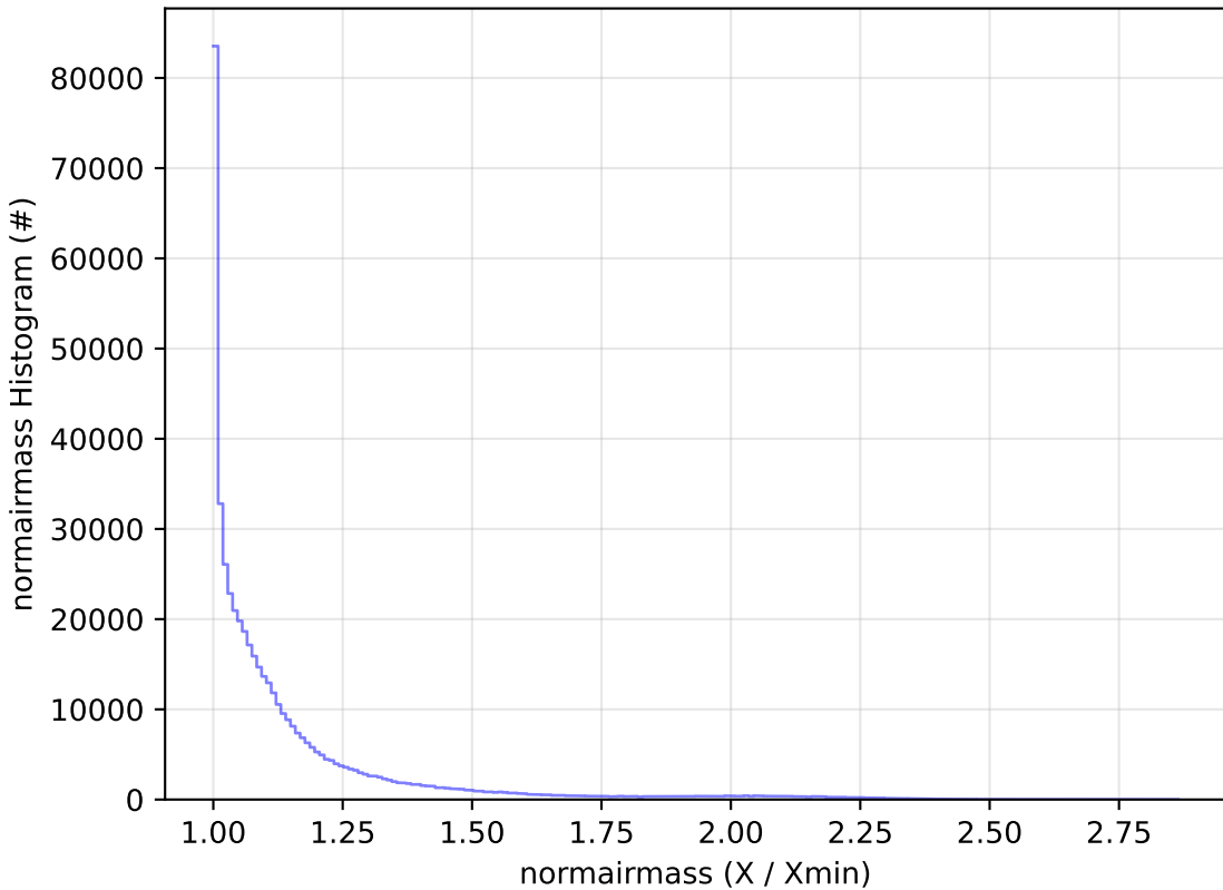
ddf_acor_sf25_lsf40_lsr10_v3.4_10yrs WFD r band: normairmass Histogram
