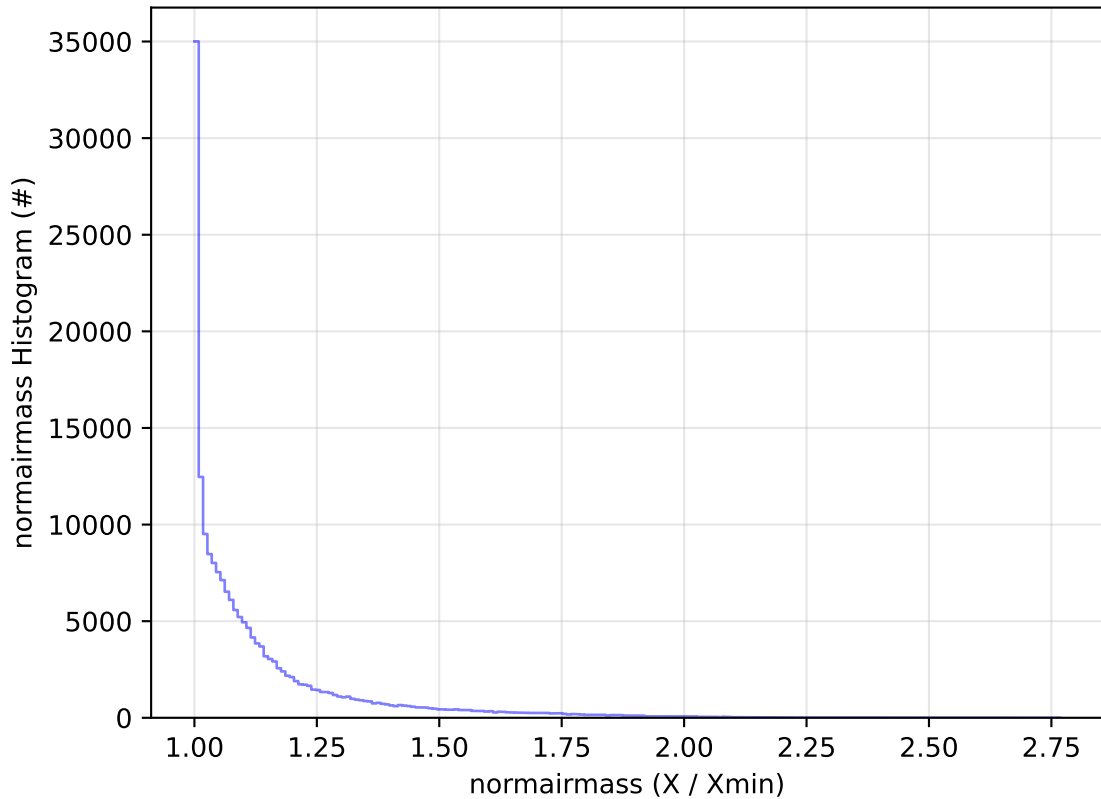
ddf_acor_sf25_lsf40_lsr10_v3.4_10yrs WFD g band: normairmass Histogram
