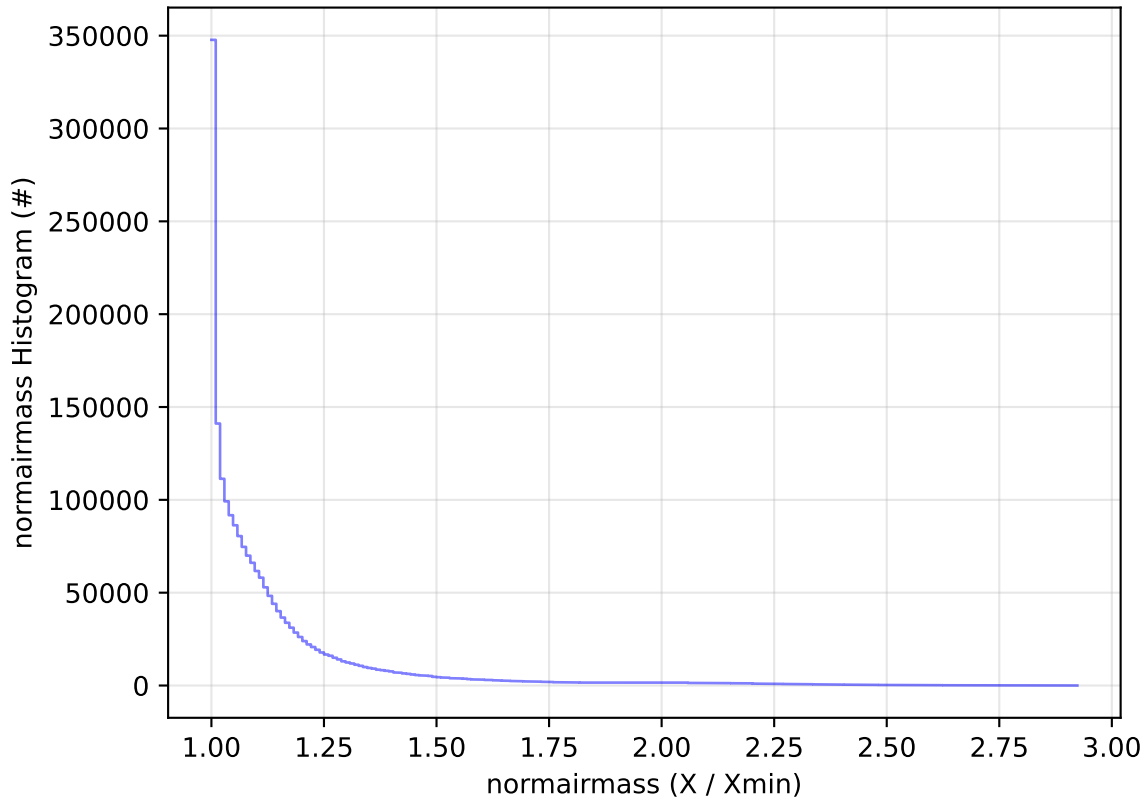
ddf_acor_sf25_lsf40_lsr10_v3.4_10yrs WFD all bands: normairmass Histogram
