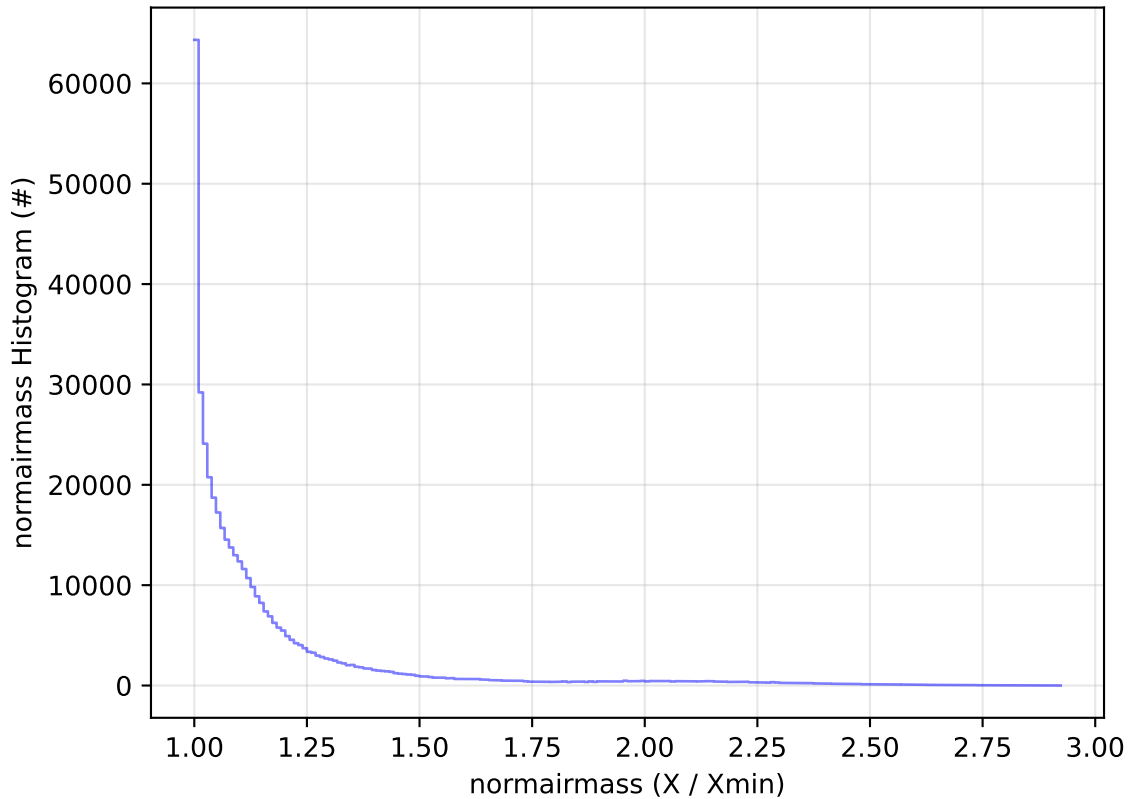
ddf_acor_sf25_lsf40_lsr10_v3.4_10yrs All sky z band: normairmass Histogram
