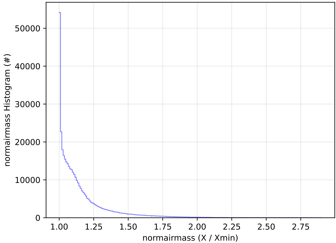
ddf_acor_sf25_lsf40_lsr10_v3.4_10yrs All sky y band: normairmass Histogram
