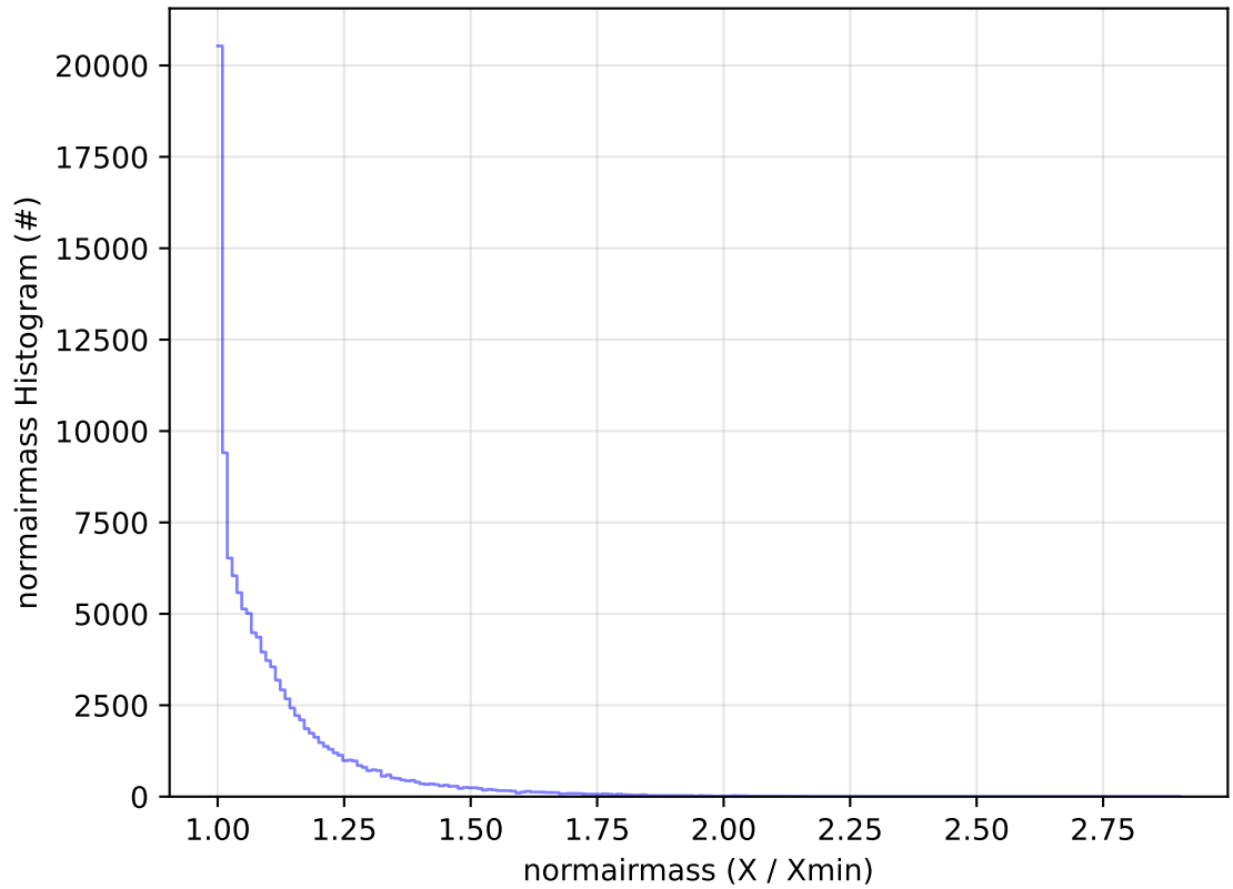
ddf_acor_sf25_lsf40_lsr10_v3.4_10yrs All sky u band: normairmass Histogram
