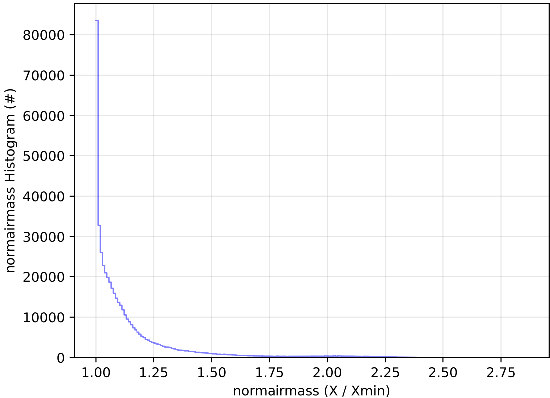
ddf_acor_sf25_lsf40_lsr10_v3.4_10yrs All sky r band: normairmass Histogram
