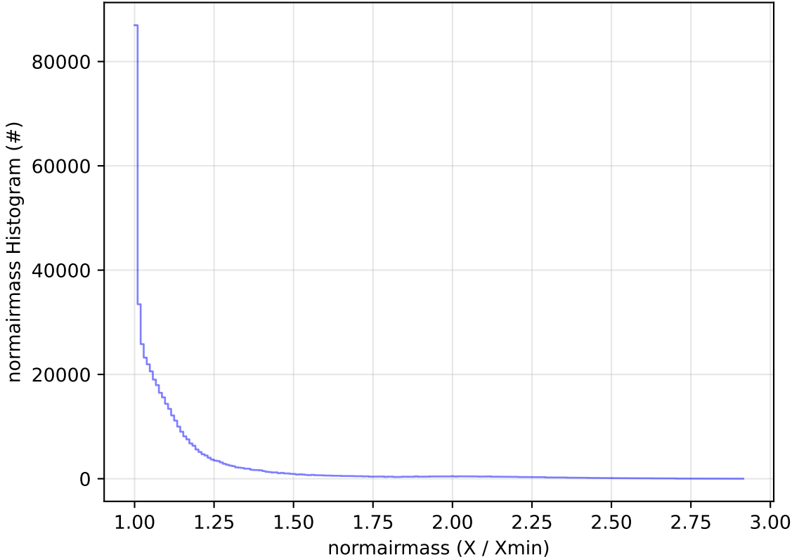
ddf_acor_sf25_lsf40_lsr10_v3.4_10yrs All sky i band: normairmass Histogram
