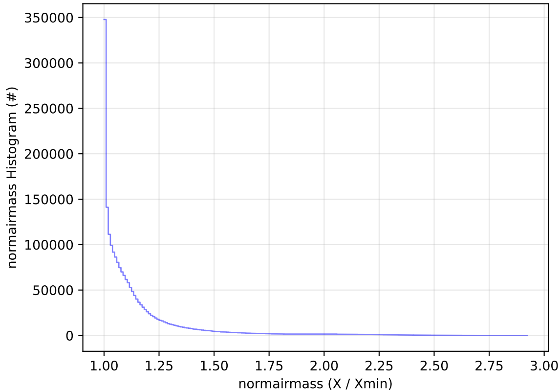
ddf_acor_sf25_lsf40_lsr10_v3.4_10yrs All sky all bands: normairmass Histogram
