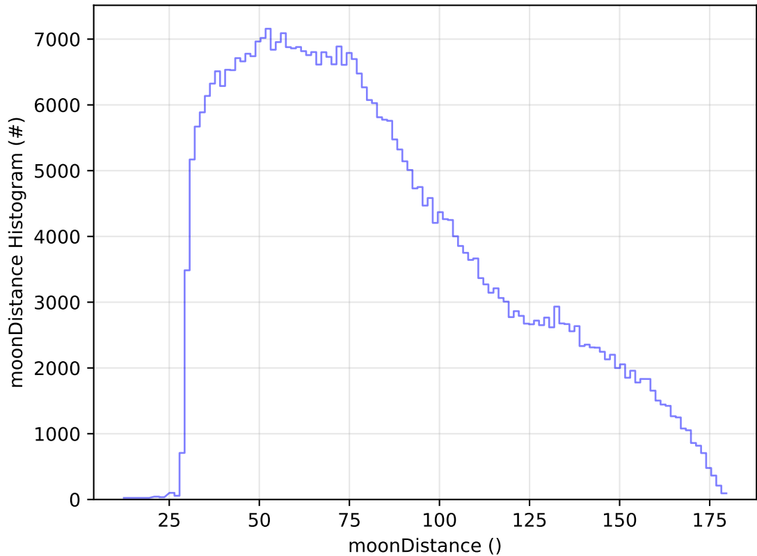
ddf_acor_sf25_Isf40_Isr10_v3.4_10yrs WFD z band: moonDistance Histogram
