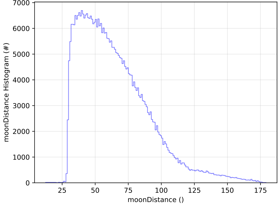
ddf_acor_sf25_Isf40_Isr10_v3.4_10yrs WFD y band: moonDistance Histogram
