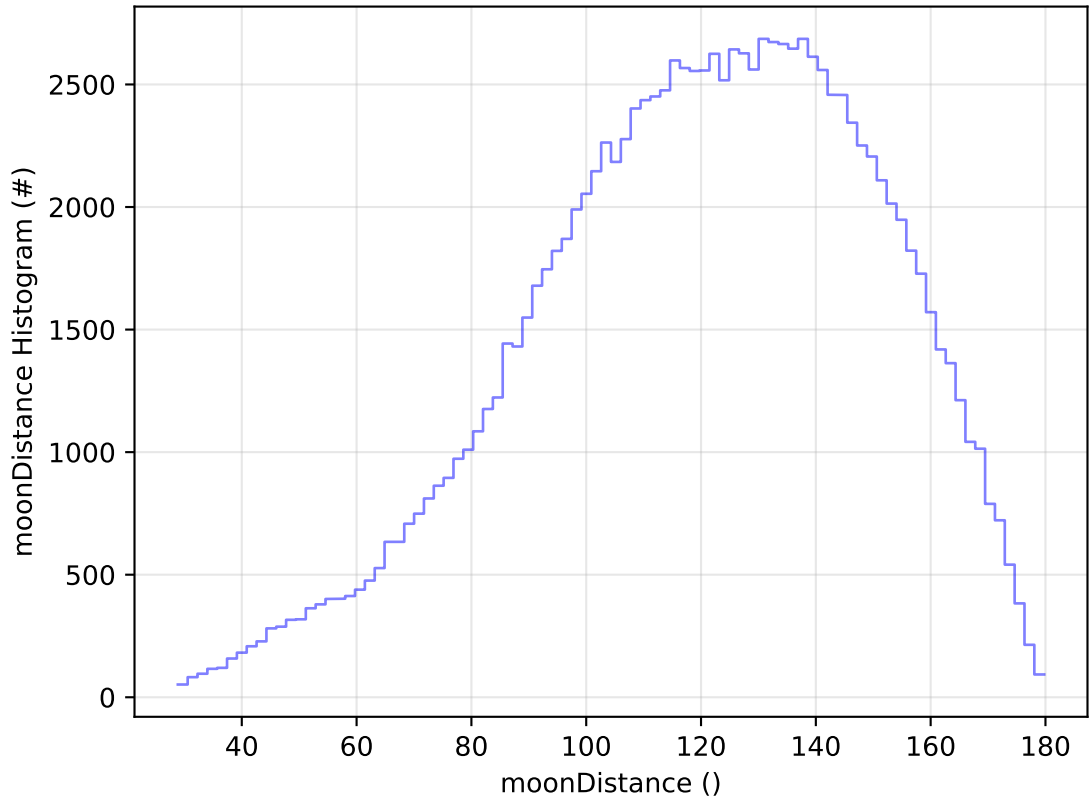
ddf_acor_sf25_lsf40_lsr10_v3.4_10yrs WFD u band: moonDistance Histogram
