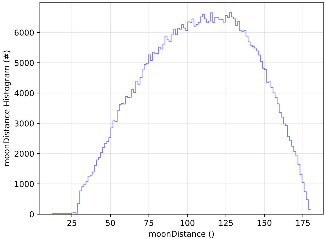
ddf_acor_sf25_lsf40_lsr10_v3.4_10yrs WFD r band: moonDistance Histogram
