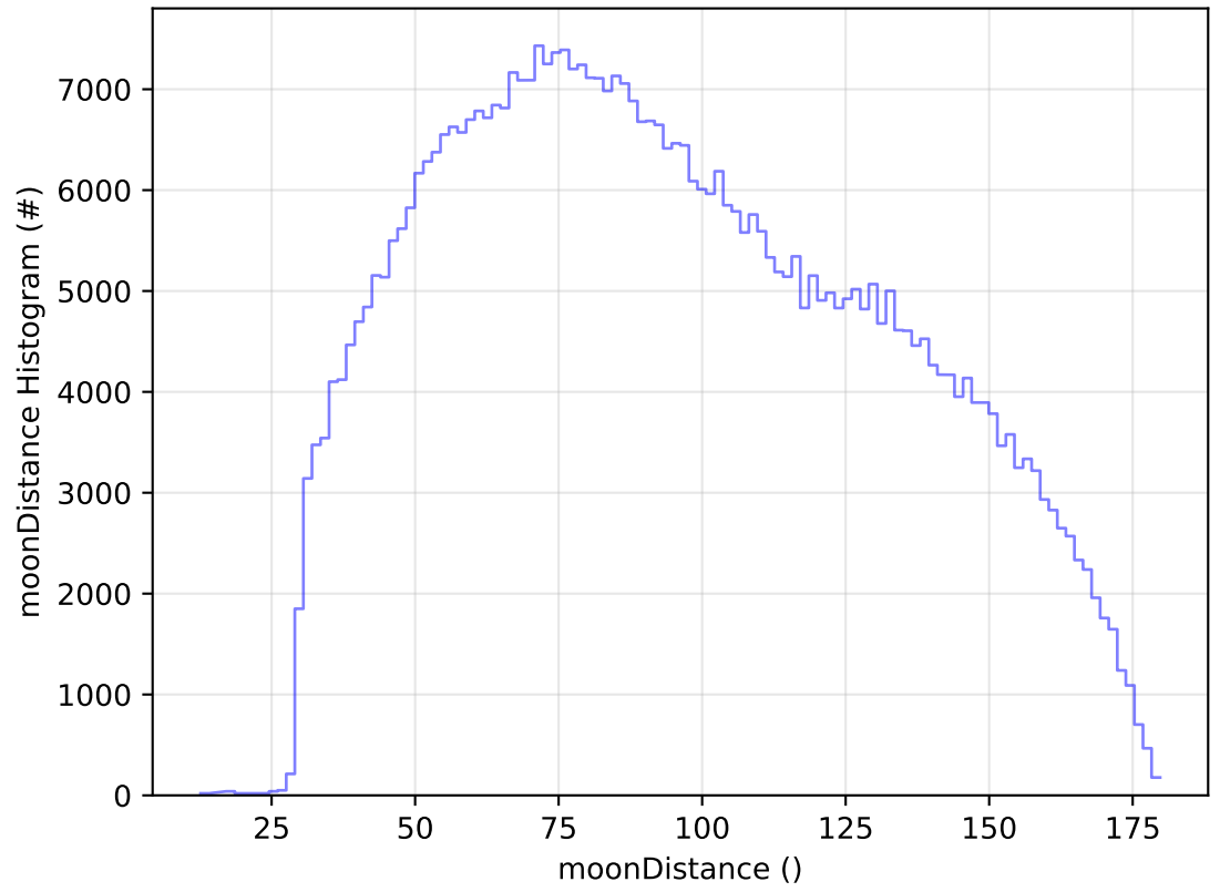
ddf_acor_sf25_lsf40_lsr10_v3.4_10yrs WFD i band: moonDistance Histogram
