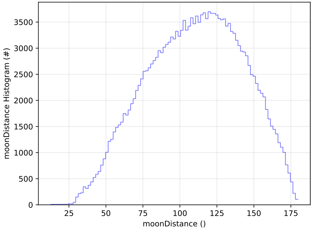
ddf_acor_sf25_lsf40_lsr10_v3.4_10yrs WFD g band: moonDistance Histogram
