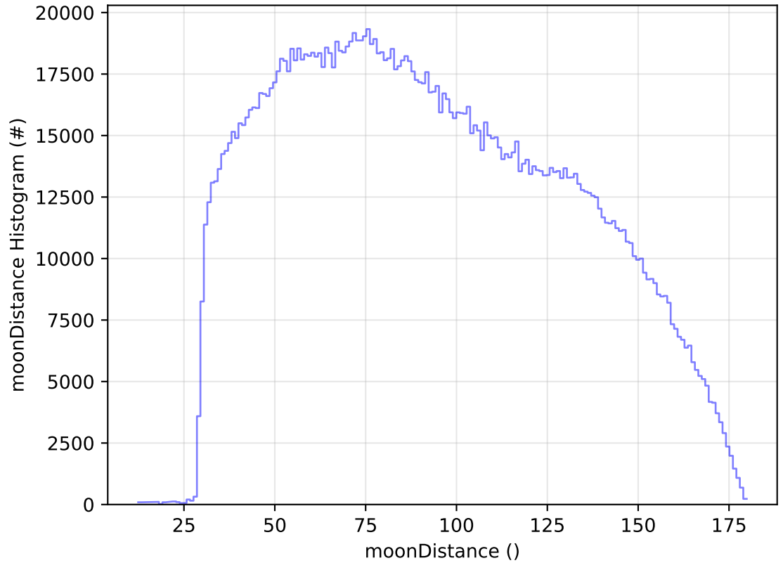
ddf_acor_sf25_lsf40_lsr10_v3.4_10yrs WFD all bands: moonDistance Histogram
