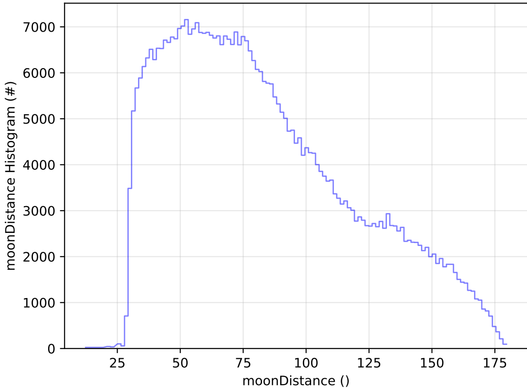
ddf_acor_sf25_lsf40_lsr10_v3.4_10yrs All sky z band: moonDistance Histogram
