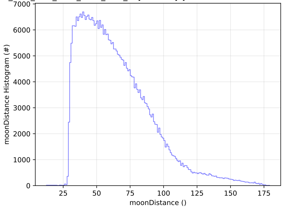
ddf_acor_sf25_lsf40_lsr10_v3.4_10yrs All sky y band: moonDistance Histogram
