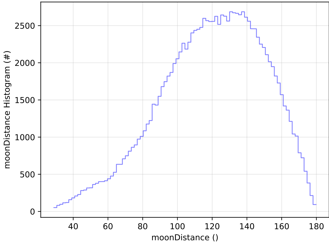
ddf_acor_sf25_lsf40_lsr10_v3.4_10yrs All sky u band: moonDistance Histogram
