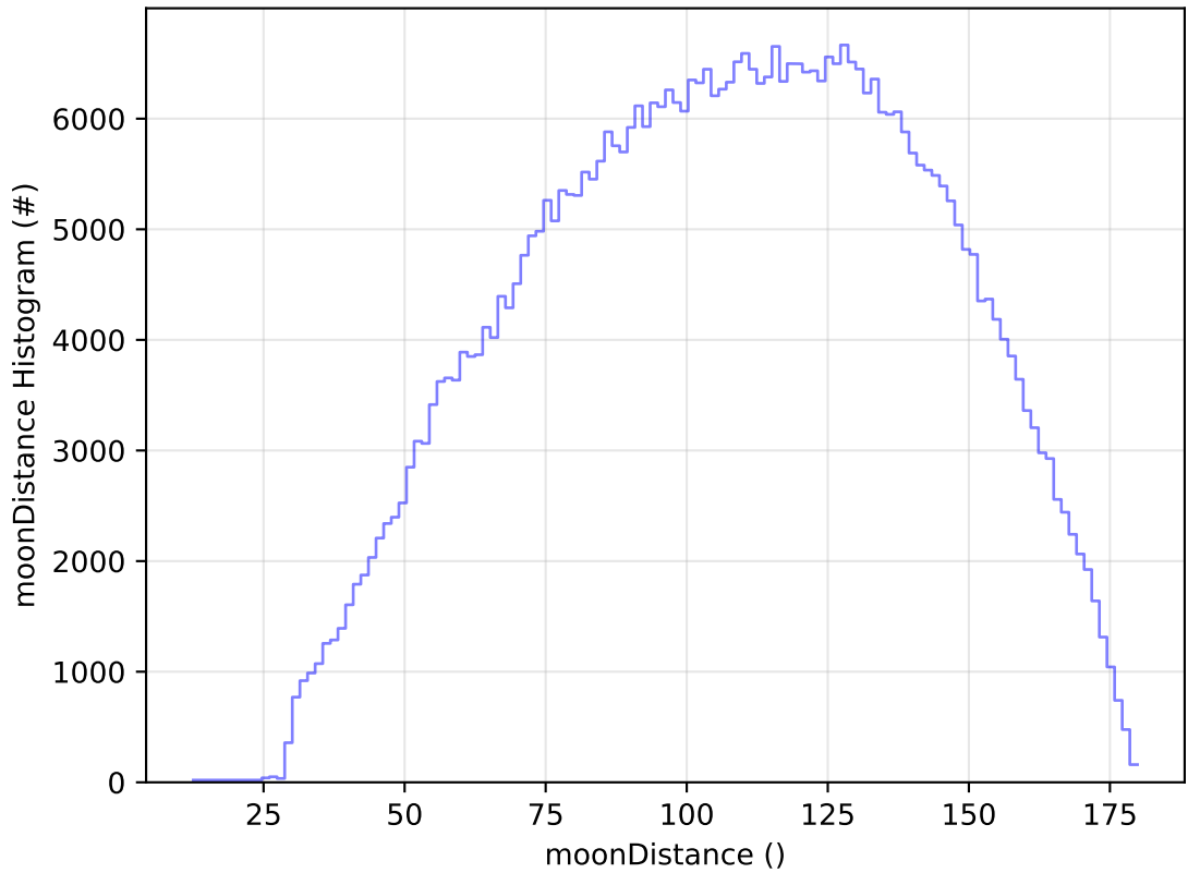
ddf_acor_sf25_lsf40_lsr10_v3.4_10yrs All sky r band: moonDistance Histogram
