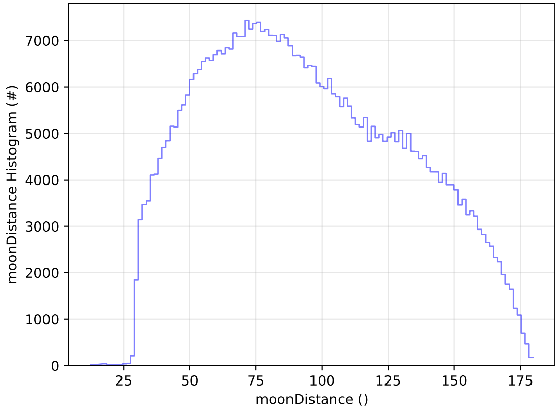
ddf_acor_sf25_lsf40_lsr10_v3.4_10yrs All sky i band: moonDistance Histogram
