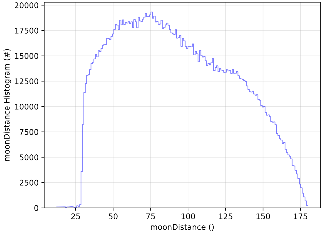
ddf_acor_sf25_lsf40_lsr10_v3.4_10yrs All sky all bands: moonDistance Histogram
