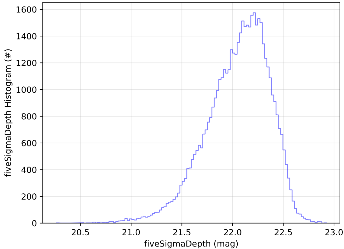
ddf_acor_sf25_lsf40_lsr10_v3.4_10yrs Yr 1 y band: fiveSigmaDepth Histogram
