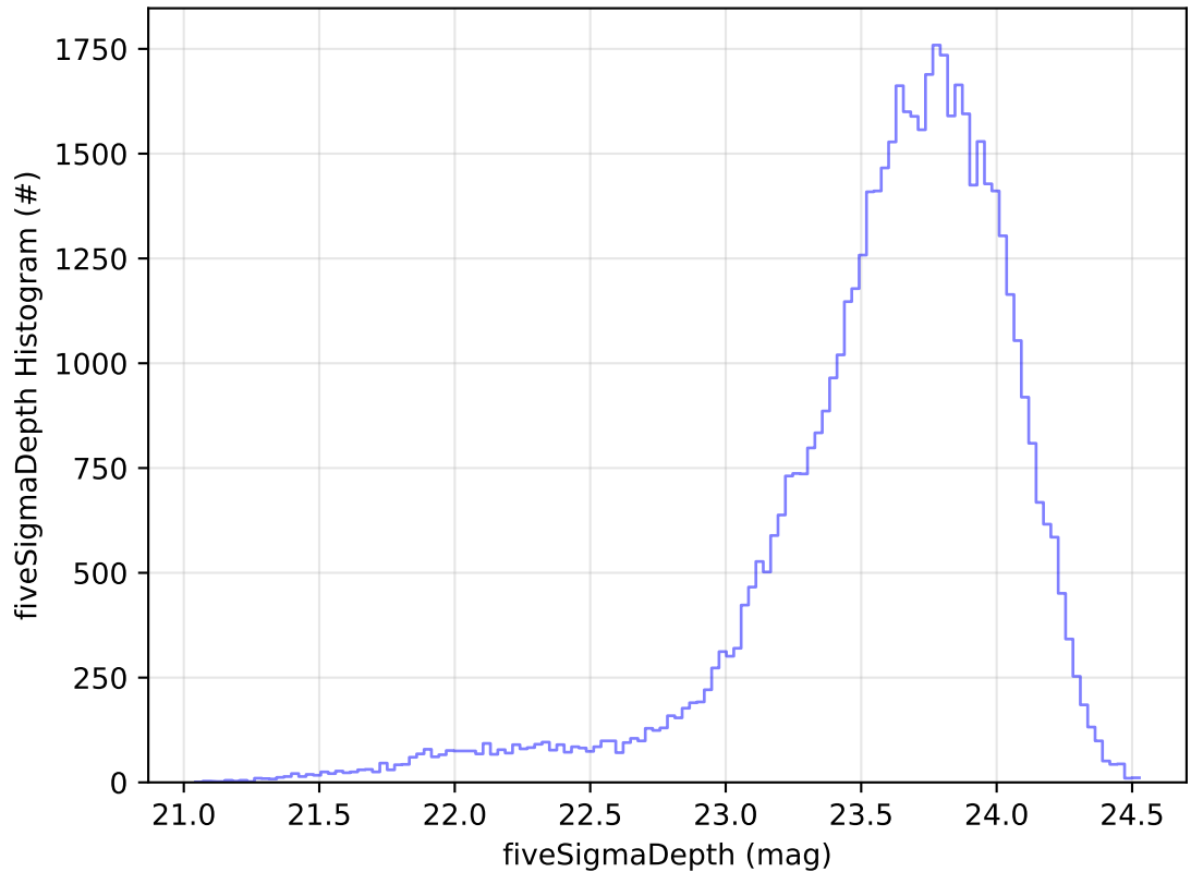
ddf_acor_sf25_lsf40_lsr10_v3.4_10yrs Yr 1 i band: fiveSigmaDepth Histogram
