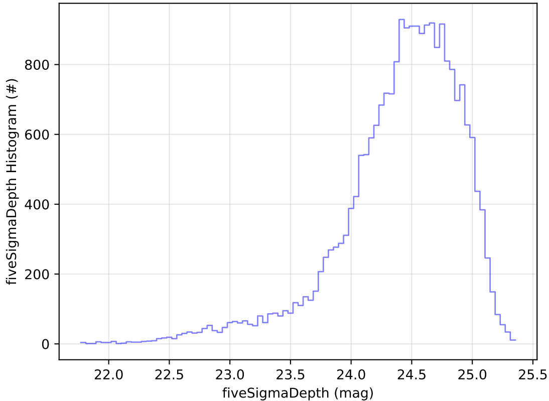
ddf_acor_sf25_lsf40_lsr10_v3.4_10yrs Yr 1 g band: fiveSigmaDepth Histogram
