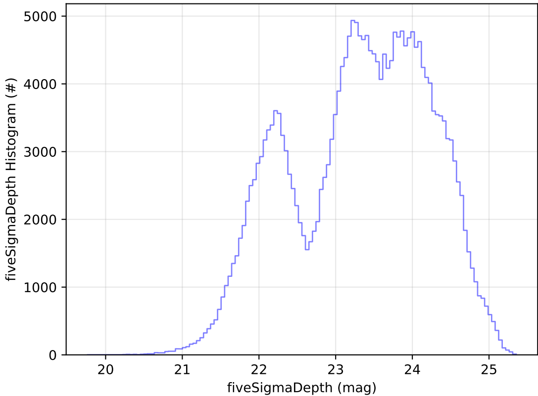
ddf_acor_sf25_lsf40_lsr10_v3.4_10yrs Yr 1 all bands: fiveSigmaDepth Histogram
