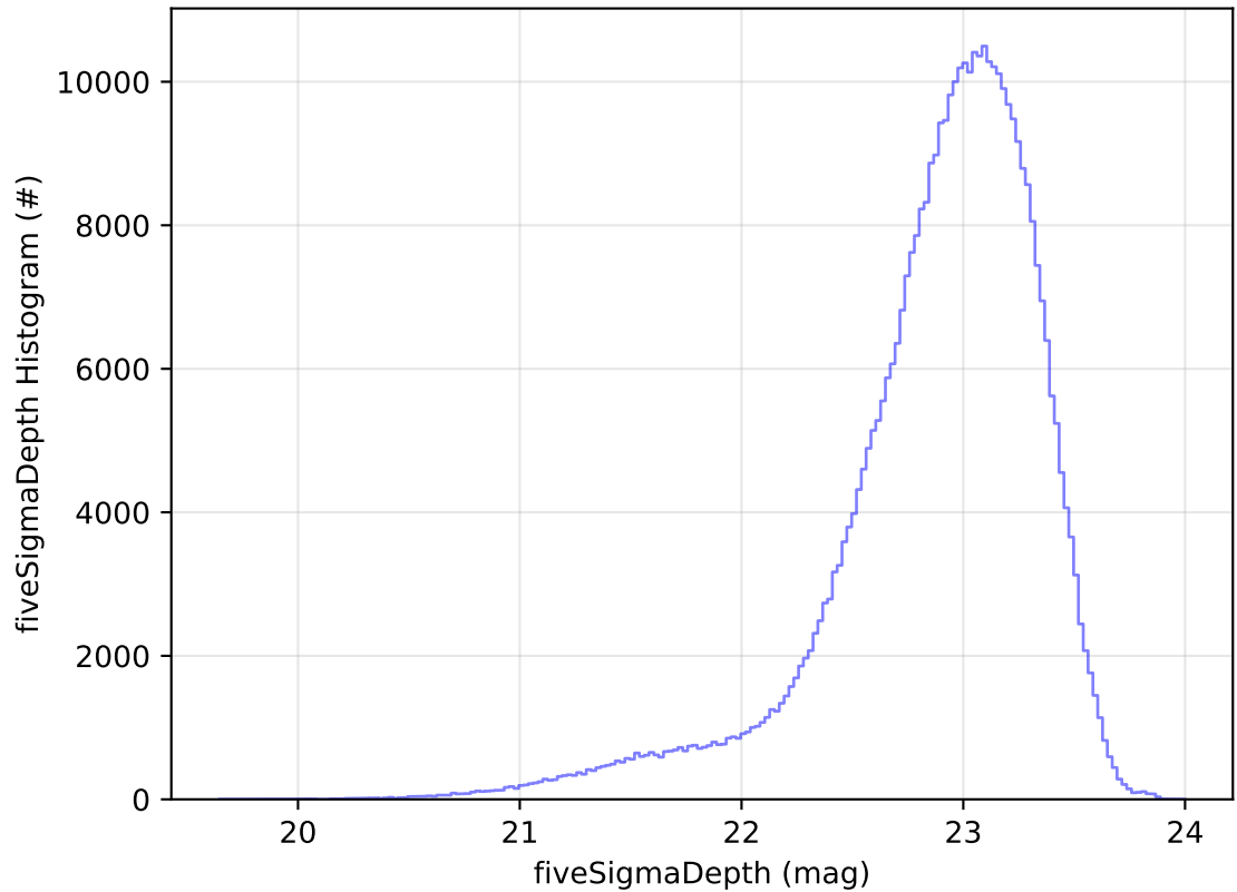
ddf_acor_sf25_lsf40_lsr10_v3.4_10yrs WFD z band: fiveSigmaDepth Histogram
