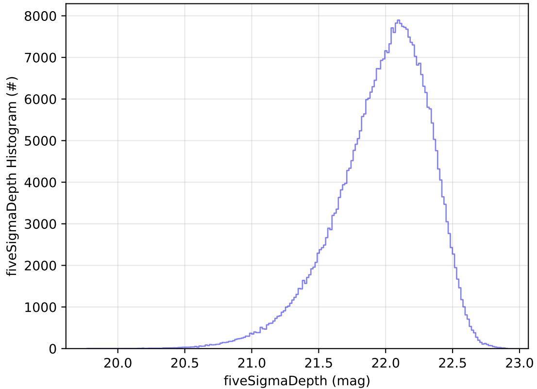
ddf_acor_sf25_lsf40_lsr10_v3.4_10yrs WFD y band: fiveSigmaDepth Histogram
