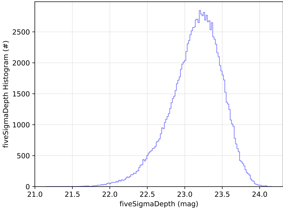
ddf_acor_sf25_lsf40_lsr10_v3.4_10yrs WFD u band: fiveSigmaDepth Histogram
